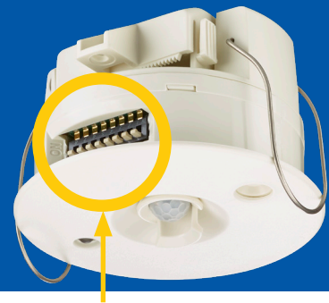
DIP switches
